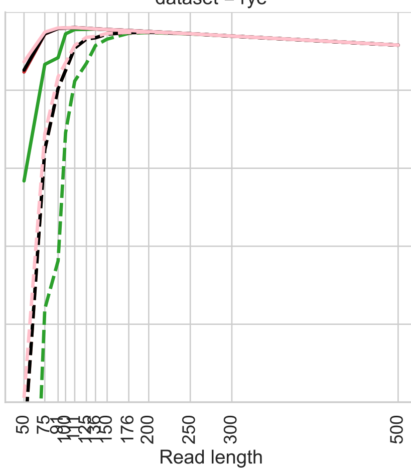
dataset = rye
