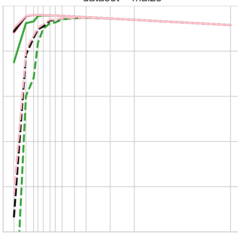
dataset = maize
